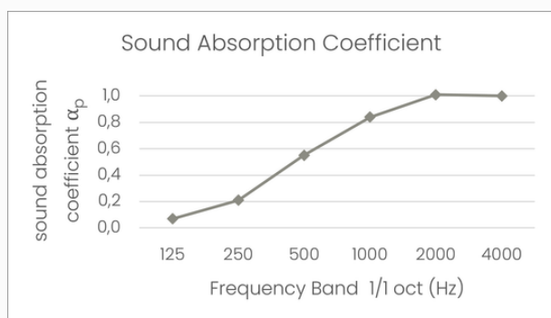
PET felt (25 mm thick) – direct mounting
