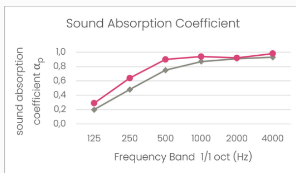
PET felt (40 mm thick) – direct mounting PET felt (40 mm thick) – 50 mm air cavity
