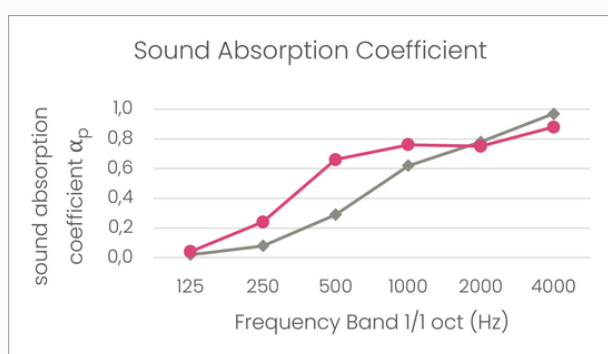
PET felt (9 mm thick) – direct mounting PET felt (9 mm thick) – 50 mm air cavity
